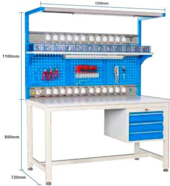
Electrician and Electronics Workbench 3-25.102
