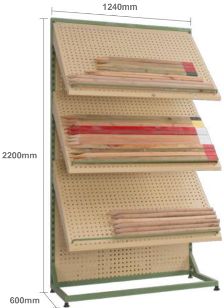
Equipment Rack N-80.112
