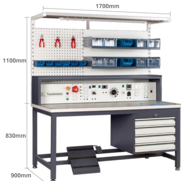
Electrician and Electronics Workbench
