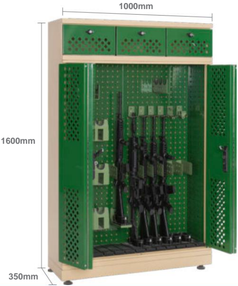
Equipment Cabinet N-80.120
