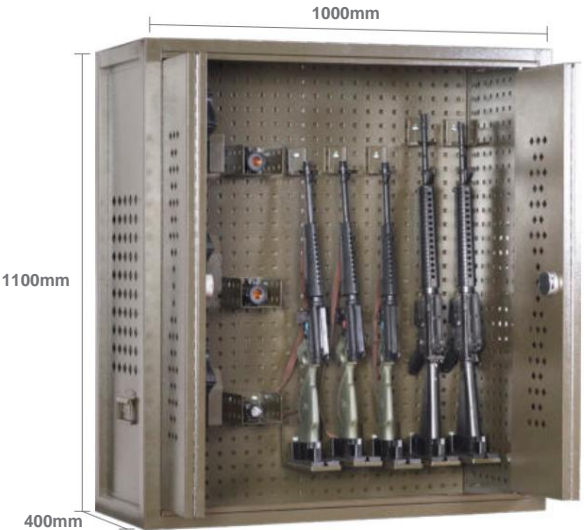
Equipment Rack N-80.132
