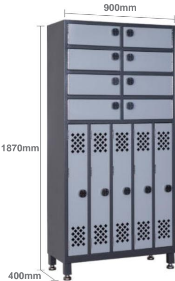
Equipment Cabinet N-80.122
