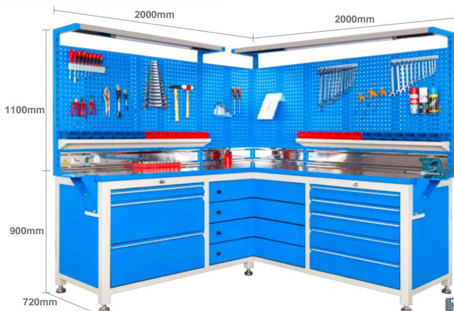
L Profile Work Bench A-15,774
