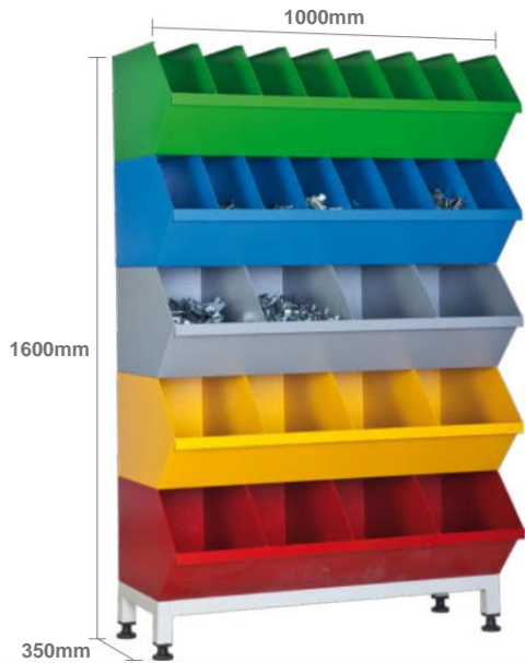
Fittings Material Stock Rack L-65.146
