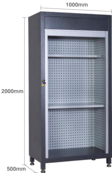
Equipment Cabinet N-80.106
