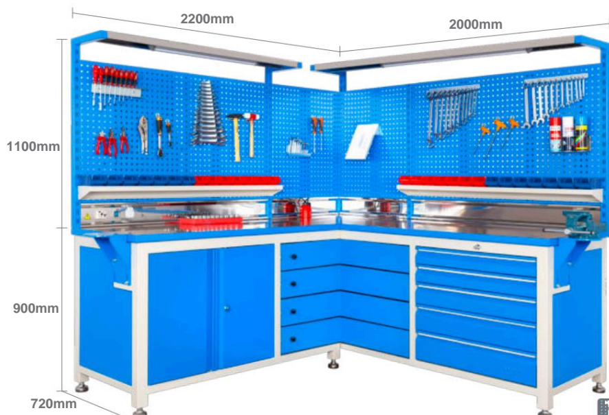
L Profile Work Bench A-15,772
