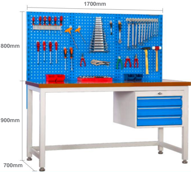
Work Bench A-16.152
