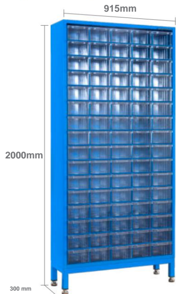
One Way Drawer Box Stand P-90.352
